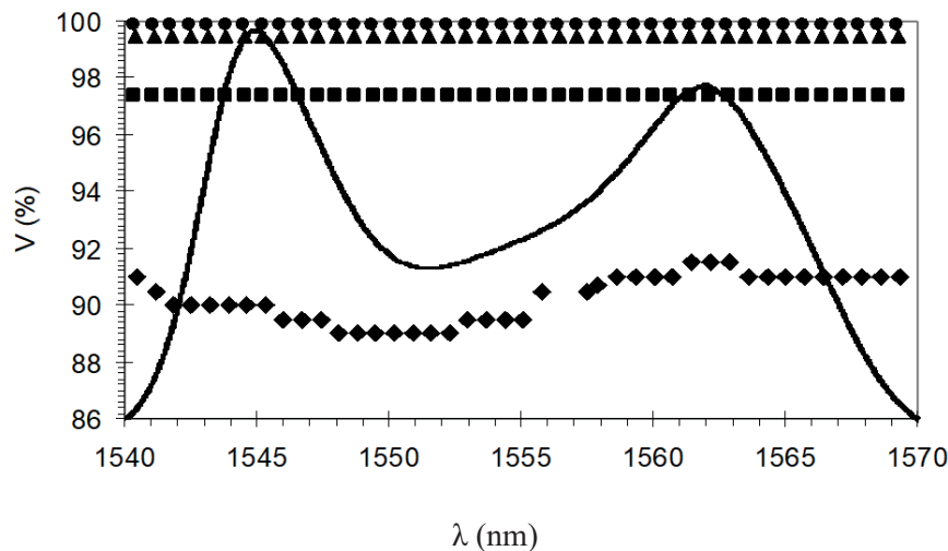
Fig.1. The dependence of visibility on the wavelength.
